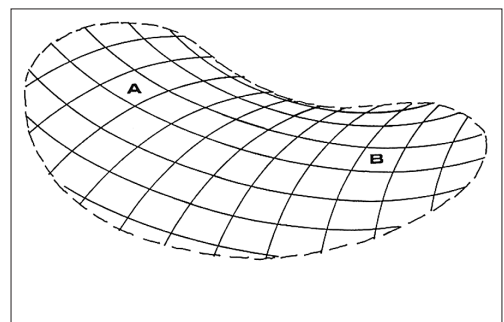
Fig. 2.4 Anti-clastic surface
